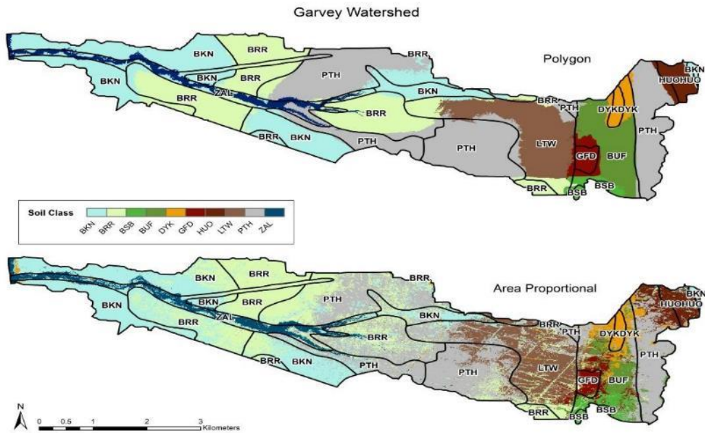
Figure 40 : Disaggregated Soil Series Maps of Garvey Glenn Creek Watershed at 30 m resolution.
