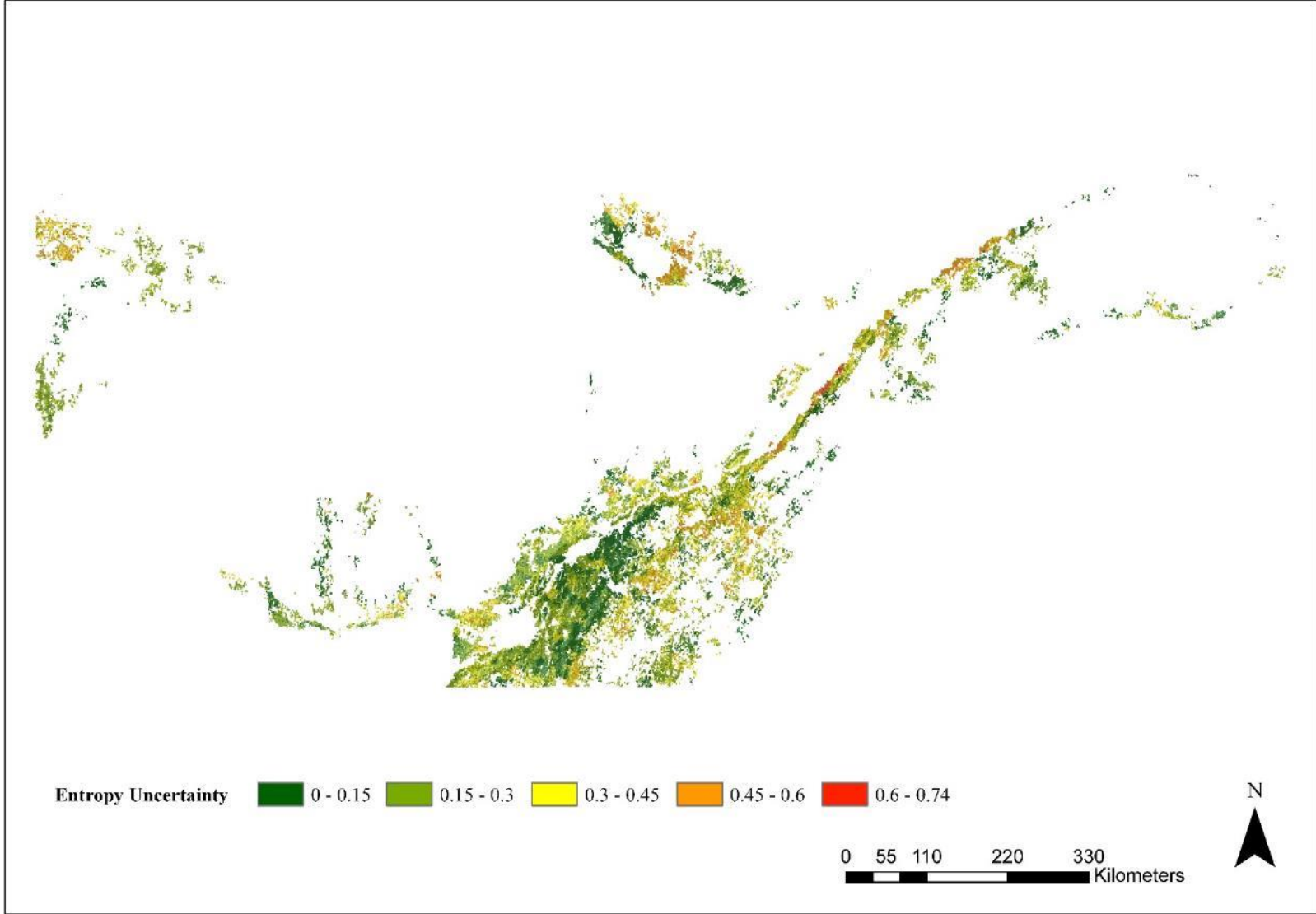
Figure 59 : Entropy Uncertainty of Disaggregated Soil Organic Matter (%) Map of Quebec using DSMART.
