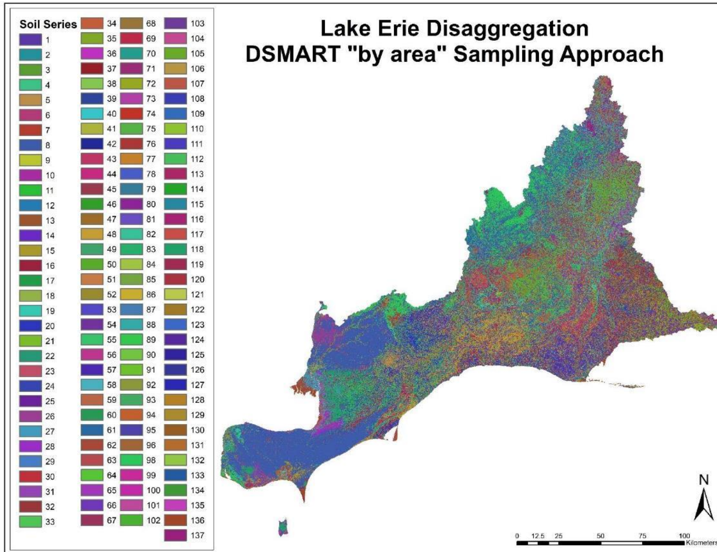
Figure 49 : Disaggregated Soil Series Map of Lake Erie Basin at 250 m resolution ("by area" Sampling Approach in DSMART) *
