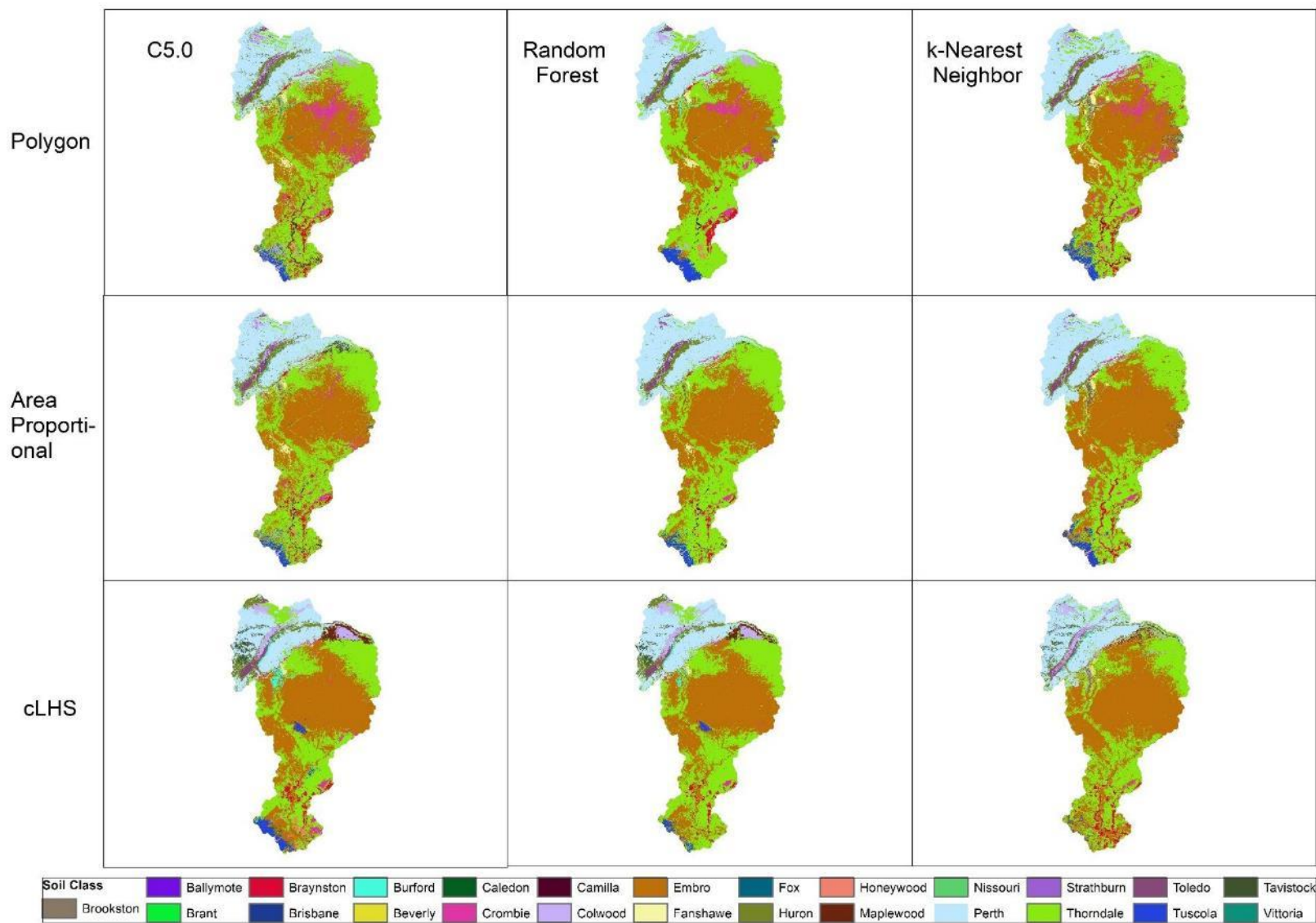
Figure 45 : Comparison of Soil Series Prediction between Different Models and Sampling Approaches in DSMART, Medway Watershed.
