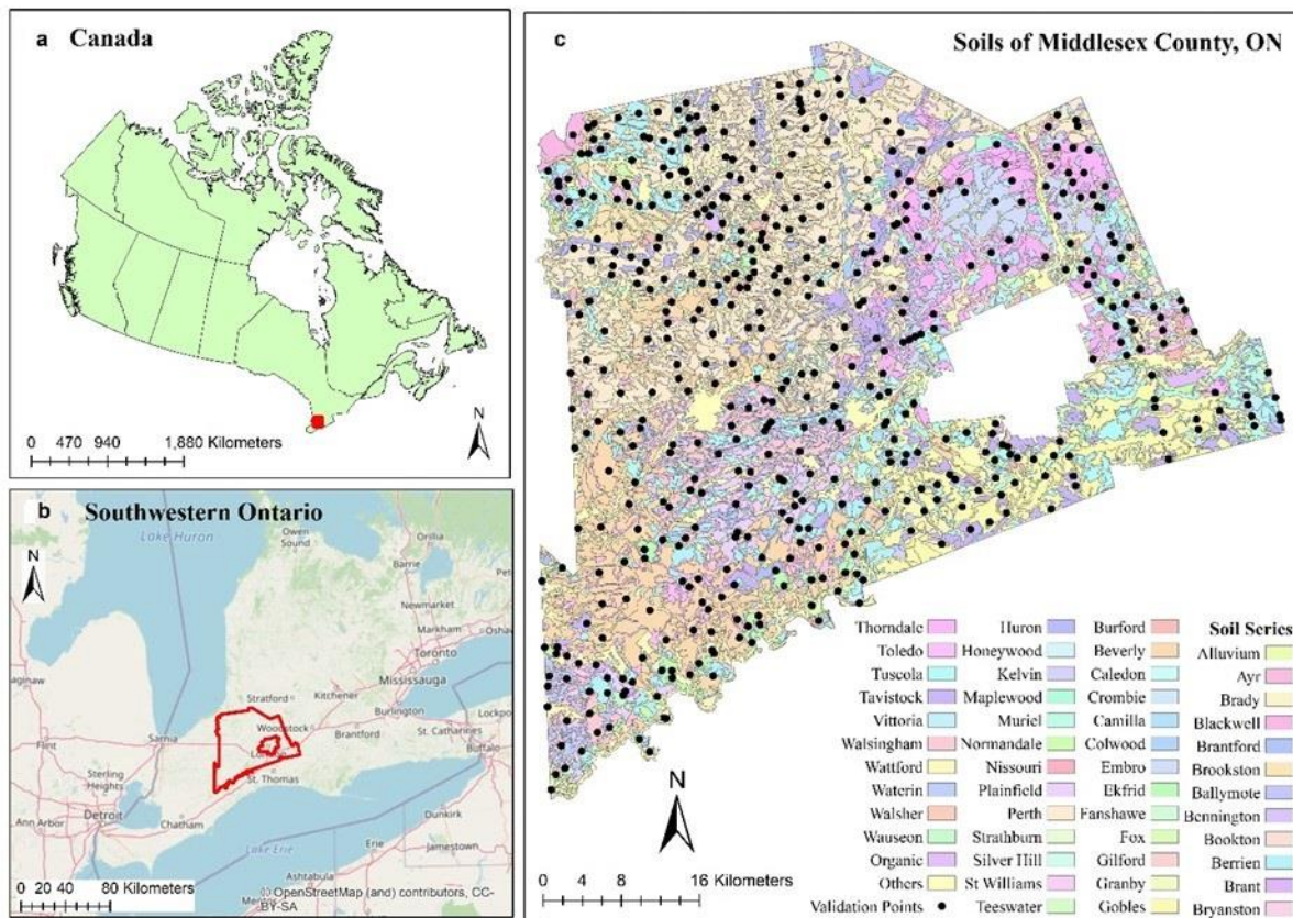
Figure 46 : Study area, Middlesex County, shown by the red dot in the map of Canada (a) and by the red boundary area Ontario and in Southwestern Ontario (b). Soil series maps of Middlesex County and validation points represented by black dots from the 1992 soil survey report of Middlesex County (c).
