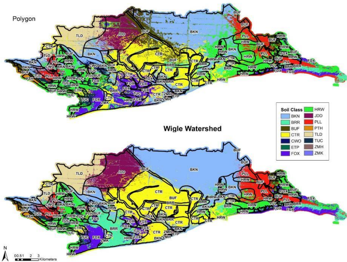
Figure 43 : Disaggregated Soil Series Maps of Wigle Creek Watershed at 30 m resolution.
