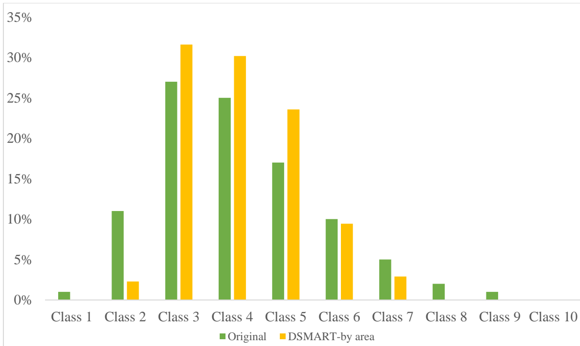
Figure 58 : Comparison between observed SOM (%) classes generated from the database compiled by IRDA and predicted SOM (%) classes from the disaggregation approach using DSMART.
