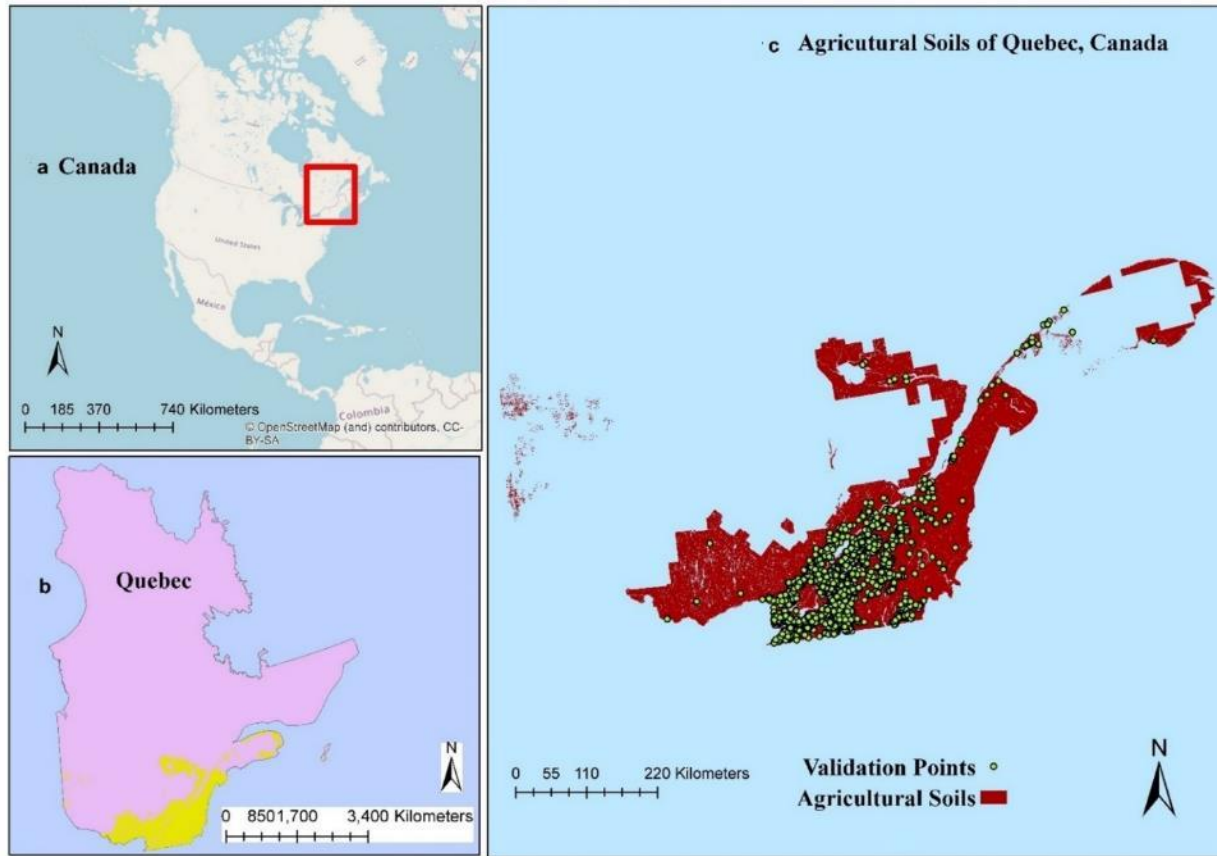
Figure 56 : The study area located in North America (a) and the agricultural soils of Quebec represented by a yellow boundary area in Quebec (b). Validation points extracted from a georeferenced private laboratory dataset are represented by green dots in the agricultural soil map of Quebec (c).
