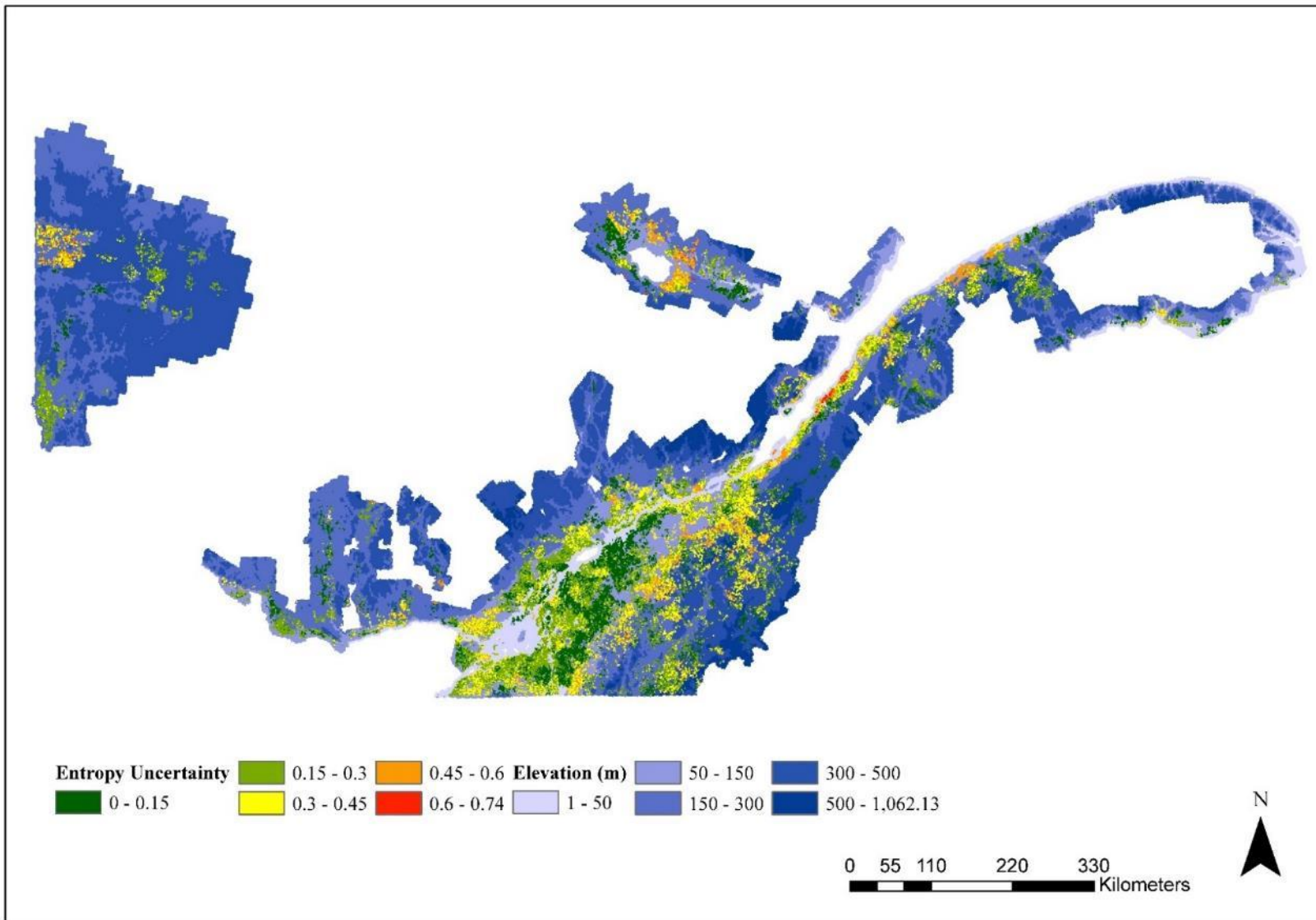
Figure 60 : Entropy Uncertainty of Disaggregated Soil Organic Matter (%) Map of Quebec using DSMART.
