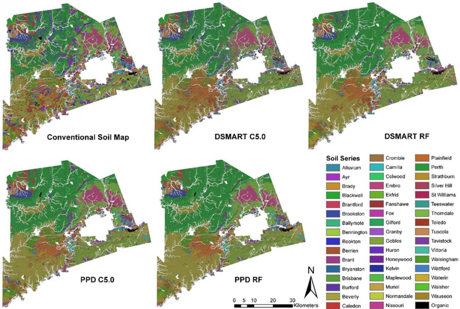
Figure 47 : Disaggregated Soil Series Map using DSMART and Pure Polygon Disaggregation of Middlesex County, ON at 50 m resolution (Area-Weighted Random Sampling Approach)
