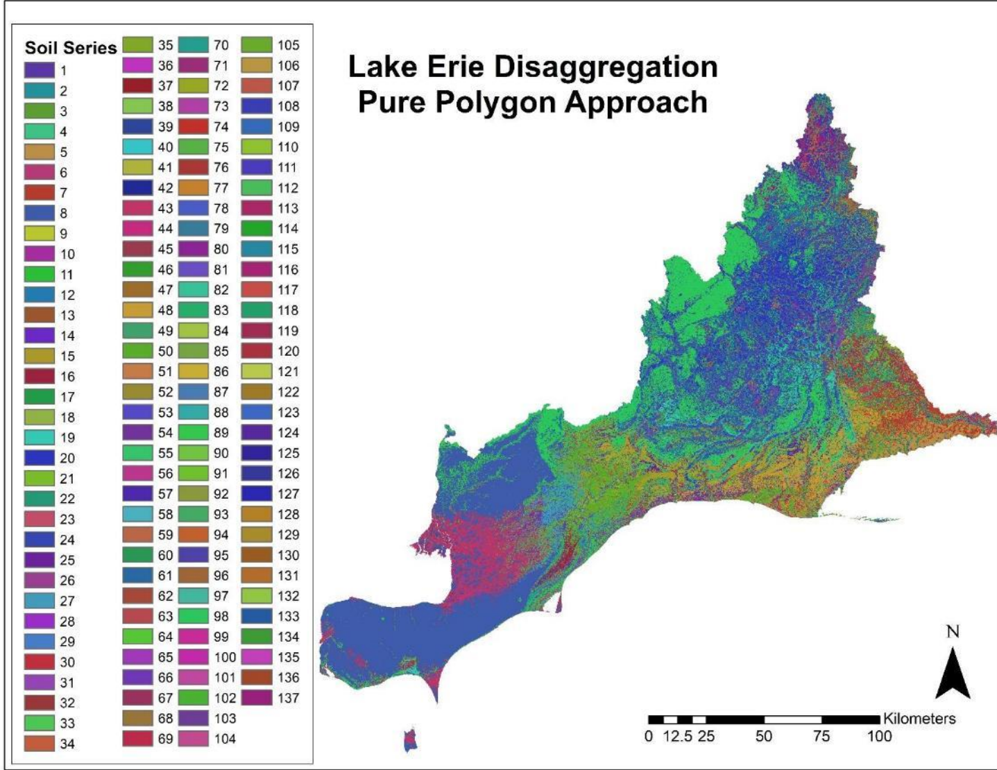
Figure 50 : Disaggregated Soil Series Map of Lake Erie Basin at 250 m resolution (Pure Polygon Approach) *
