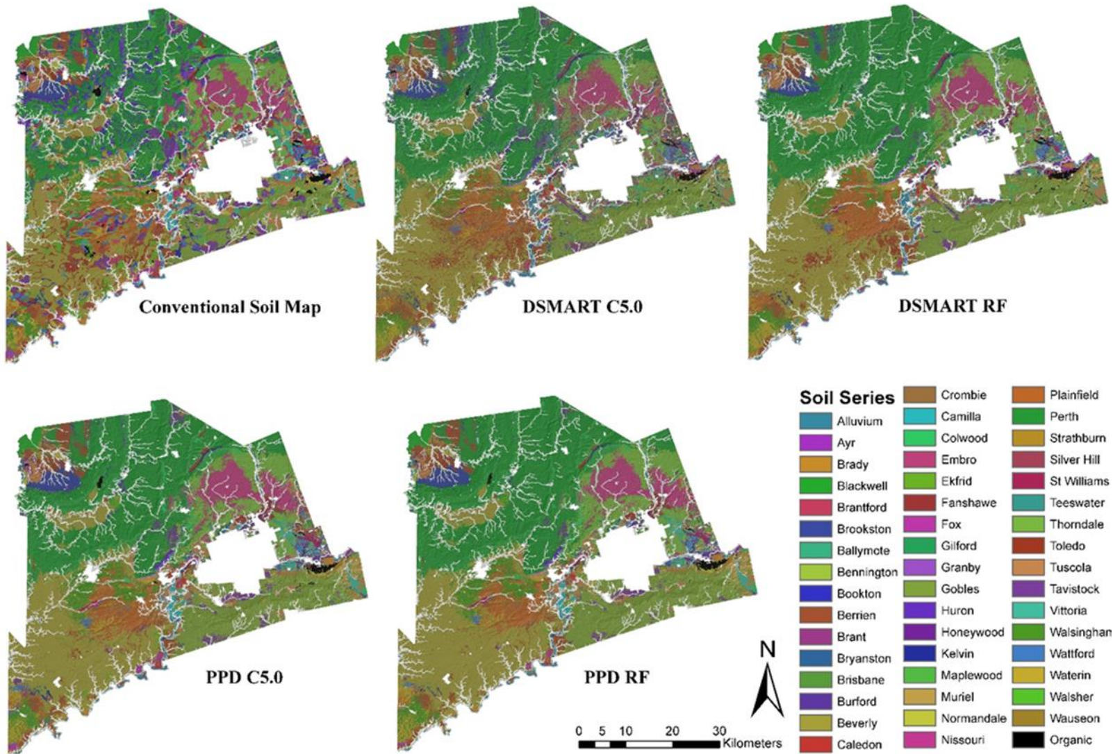
Figure 48 : Disaggregated Soil Series Map using DSMART and Pure Polygon Disaggregation of Middlesex County, ON at 50 m resolution (Conditional Latin Hypercube Sampling Approach)
