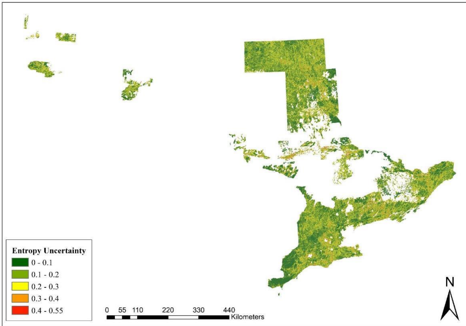
Figure 53 : Entropy uncertainty of C5.0 in Pure Polygon Disaggregation using training data produced from area-weighted random approach at a 250m spatial resolution, Ontario.
