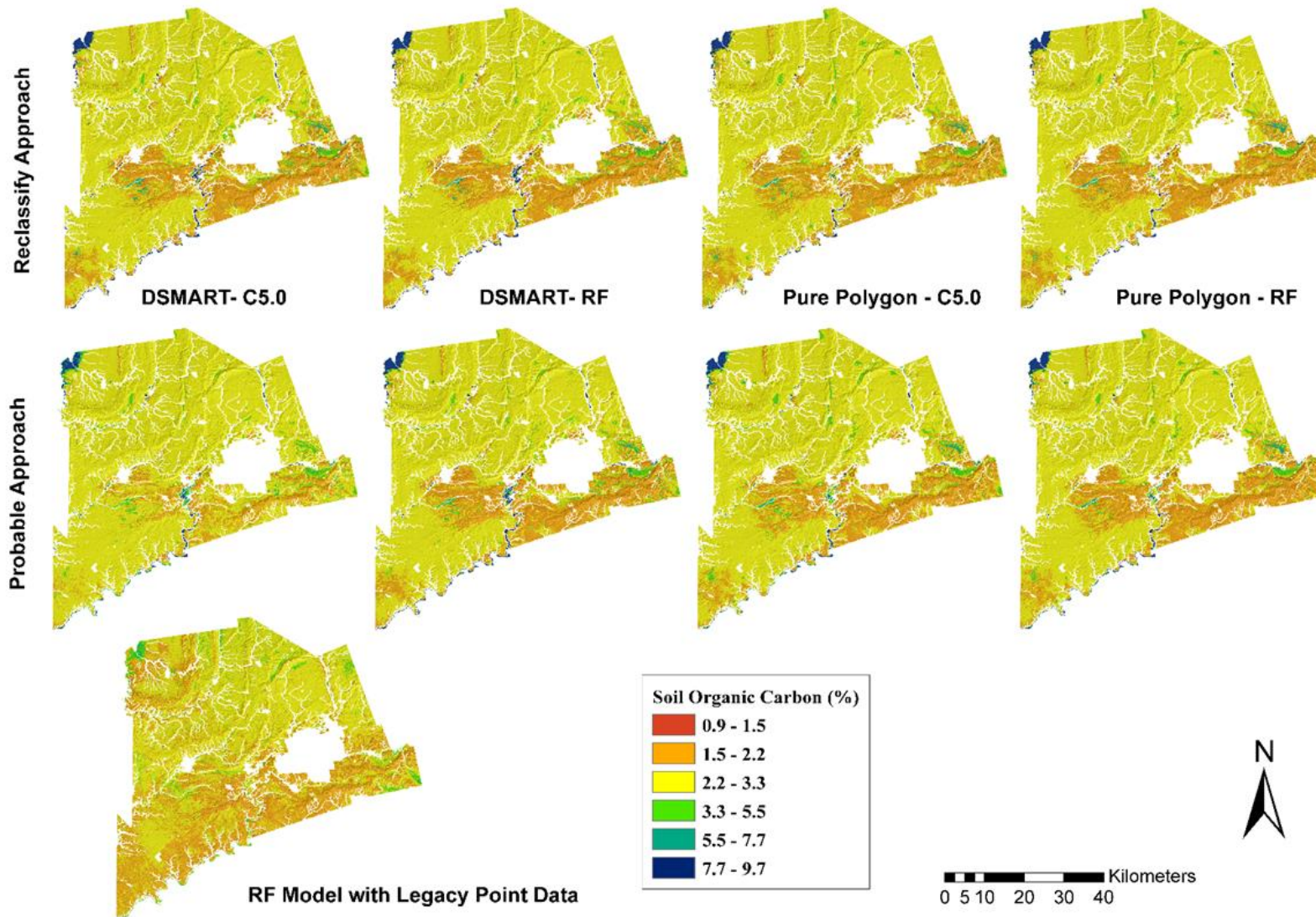
Figure 54 : Mean SOC% prediction map at 0-30 cm depth of Middlesex County using reassigned and weighted-probable models.
