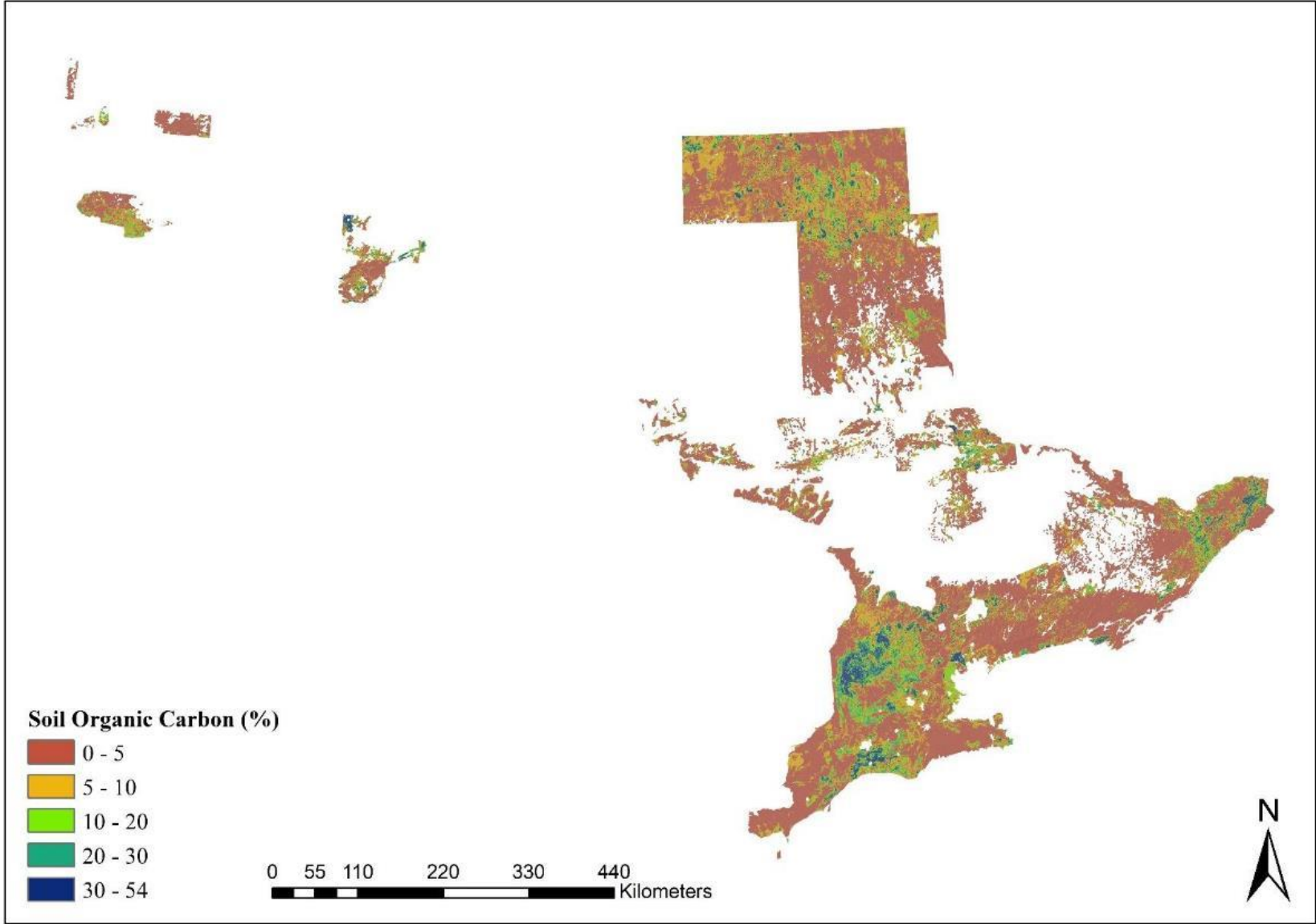
Figure 55 : Soil Organic Prediction Map of Agricultural Soils of Ontario using Probable-Classifer Approach.
