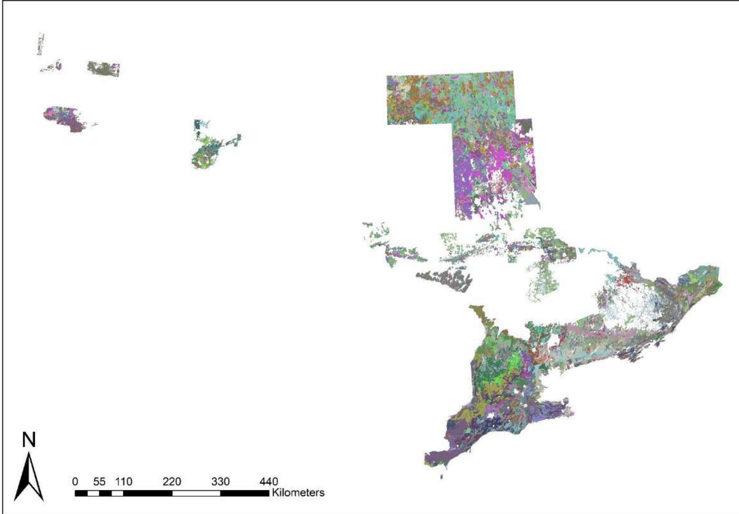
Figure 52 : Disaggregated Soil Series Map of Agricultural Soils of Ontario at 250 m resolution (Pure Polygon Approach) **
