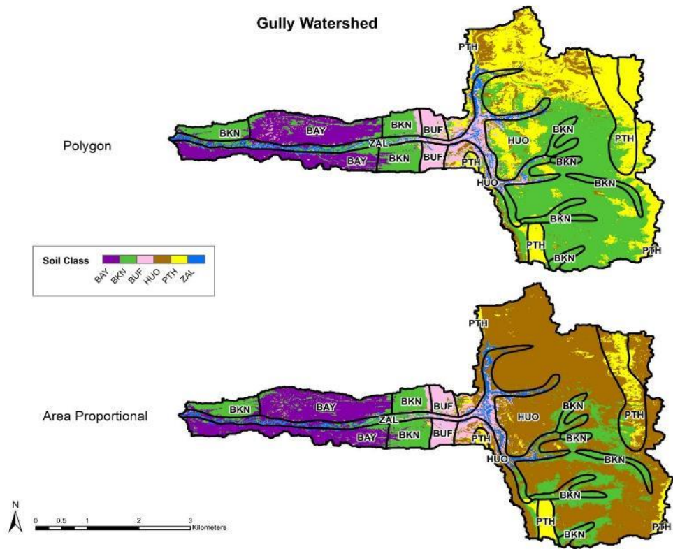
Figure 41 : Disaggregated Soil Series Maps of Gully Creek Watershed at 30 m resolution.
