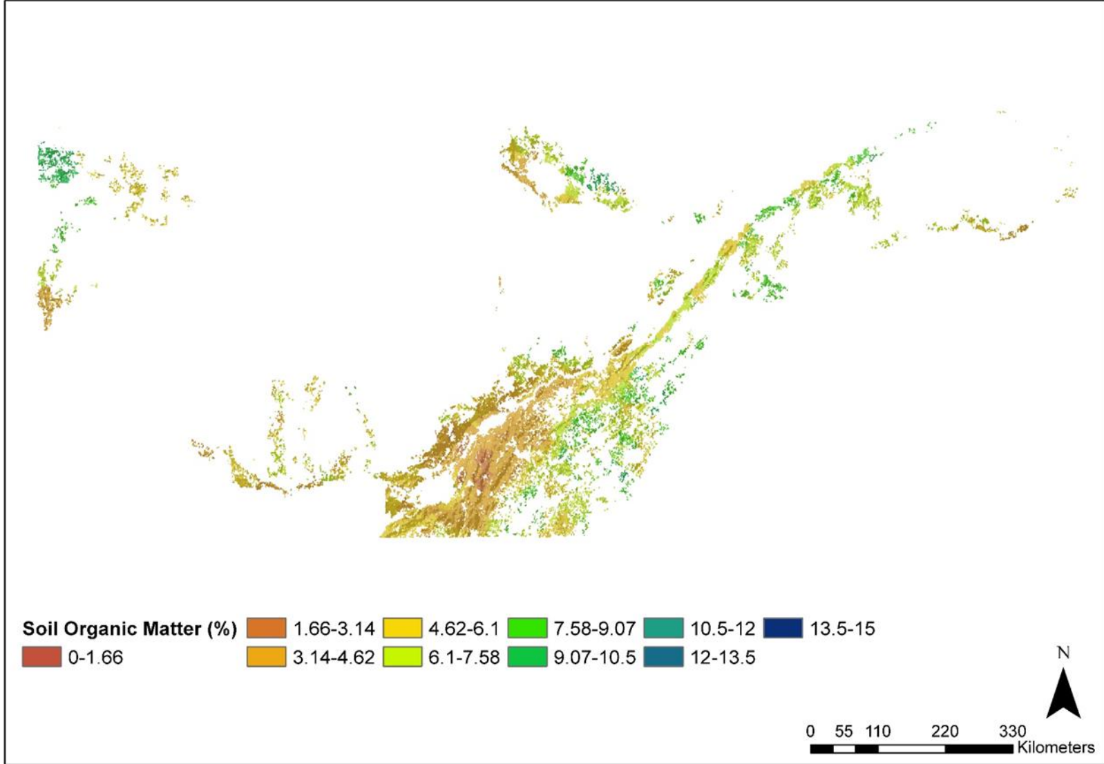
Figure 57 : Disaggregated Soil Organic Matter (%) map of Quebec agricultural soils at 250m resolution using DSMART.
