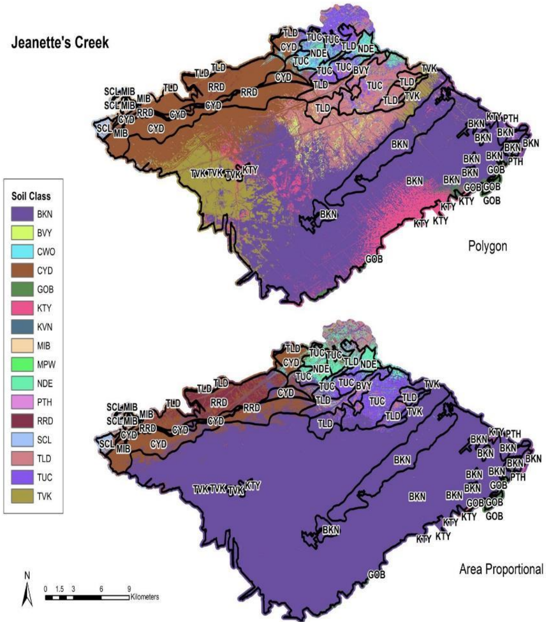
Figure 42 : Disaggregated Soil Series Maps of Jeanette's Creek Watershed at 30 m resolution.
