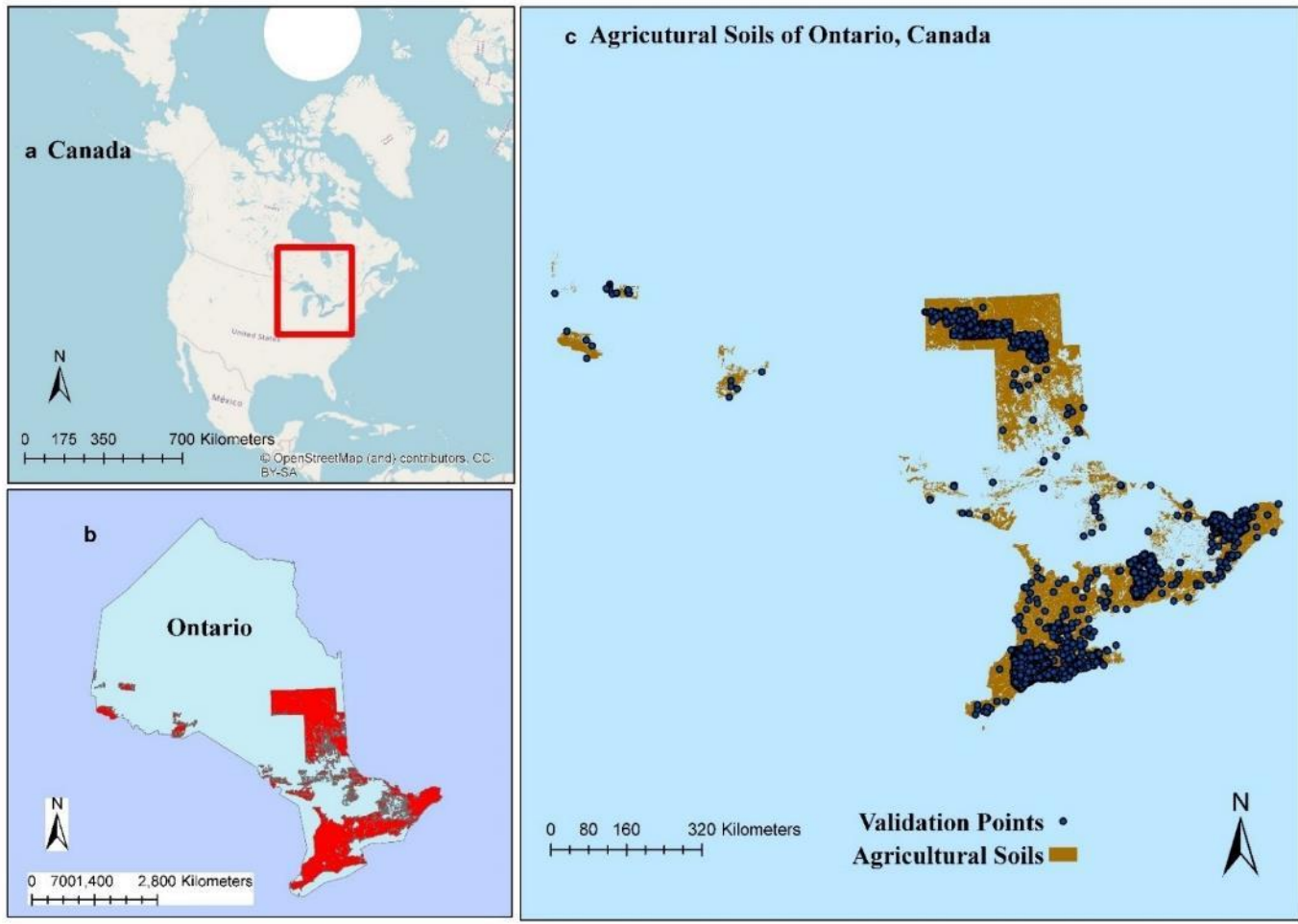
Figure 51 : The study area located in North America (a) and the soils of Ontario represented by the red boundary area in Ontario (b). Validation points extracted from the National Pedon Database are represented by blue dots in the agricultural soil map of Ontario (c).
