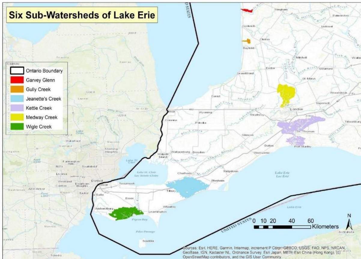
Figure 39 : Six Sub-Watersheds of Lake Erie.
